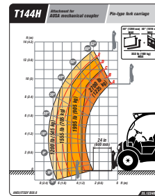
AUSA carriage
